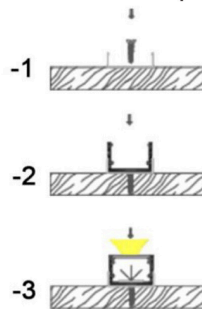
Installation steps
