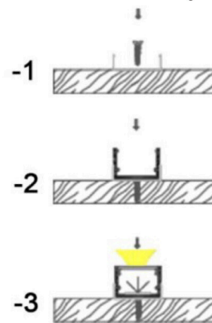
Installation steps
