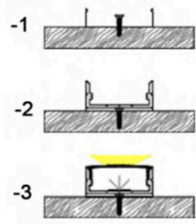
Installation steps
