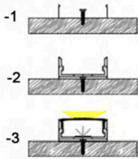
Installation steps
